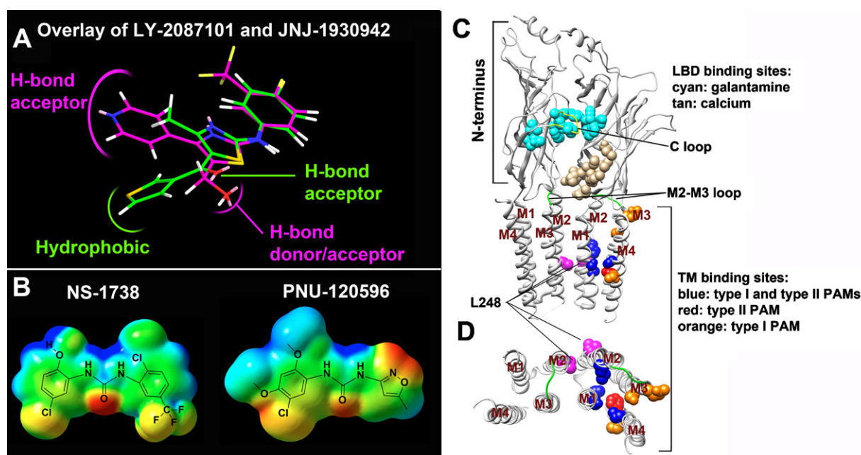
Fig. 3. \alpha 7 PAM structures and putative binding sites. A) Pharmacophore orientation comparison between LY-2087101 and JNJ-1930942. The structures of the two compounds were optimized using Chem 3D Pro v.12.0 (CambridgeSoft, Cambridge, MA): their energies were first minimized by molecular mechanics to minimum RMS gradient of 0.001 separately. Then LY-2087101 and JNJ-1930942 were overlaid on top of each other and shown in green and magenta, respectively. B) Molecular electrostatic potential surfaces of NS-1738 (left) and PNU-120596 (right). The structures of the two compounds were optimized using Gaussian09 (Gaussian, Inc., Wallingford, CT). The electrostatic potential on a total electron density isosurface ( 0.002 \text{ Bohr}/\text{\AA}^3 ) of the two compounds is displayed in GaussView (Gaussian, Inc., Wallingford, CT) with red color indicating the most negative electrostatic potential and blue color indicating the most positive electrostatic potential, respectively. The structures of the two compounds are displayed on top of each electrostatic potential surface. C) Structural domains of nAChR regulating PAM activity and/or binding. The key elements of the \alpha 7 receptor were modeled using the 2BG9 template for the transmembrane domain fused to the N-terminal extracellular domain made from the 2PGZ template. The C-loop is shown in yellow, and the M2 and M3 linker loop is shown in green. The view was made from the outside of the channel pore, and the four transmembrane helices (M1–M4) were lined clockwise as shown, putting the M2 helix toward the channel pore. Residues involved for different \alpha 7 PAMs potentiation are displayed as spheres of different colors as indicated: calcium, tan; galantamine, cyan; common residues for type I PAMs Ivermectin and LY-2087101 and the type II PAM PNU-120596, blue; residues only for Ivermectin, orange; residues only for PNU-120596, red. Leucine 248 is also shown in magenta in both subunits. D) A close-up view of the transmembrane domain, made by rotating the view in part C 90^\circ vertically away from the plane of the paper.
