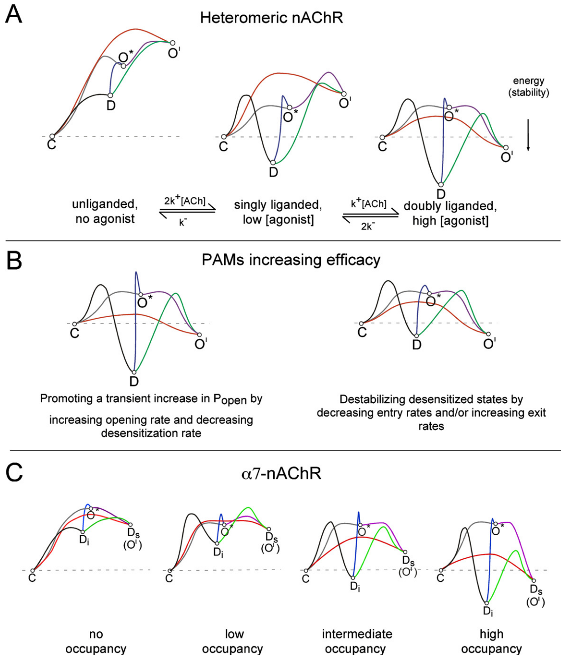
Fig. 1. The energy landscapes for nAChR state transitions. A) Hypothetical energy wells and barriers for the conformational states of heteromeric nAChR (e.g. muscle-type or neuronal \alpha 4 nAChR) as functions of the level of agonist occupancy (see description in text). Under equilibrium conditions, the distributions of receptors into the resting closed (C), brief open ( O^* ), long-lived open ( O' ), and desensitized (D) states will be determined by the relative free energy of the states (represented by vertical displacements). Dynamically, the transition rates between the states will be inversely related to the log of the energy barriers between the states. B) Two ways in which PAMs may operate on the energy profile of receptors in the doubly liganded state to increase the probability of channel opening: either transiently, after a jump in agonist concentration (left schematic) or under steady-state conditions (right schematic). C) Hypothetical scheme representing state transitions of \alpha 7 nAChR under various levels of agonist occupancy. In the absence of PAMs, \alpha 7 nAChR do not exhibit a long-lived open state, but do show a unique desensitized state ( D_s ) that is preferentially favored at higher levels of agonist occupancy. They also have an intrinsic desensitized state ( D_i ), which is analogous to the D state of heteromeric receptors (A). Very efficacious type II PAMs, such as PNU-120596, appear to either destabilize the D_s state, or hypothetically may convert it into a conducting state similar to the O' state of heteromeric receptors. This hypothesis is represented by ( O' ) symbols inserted into the panel.
