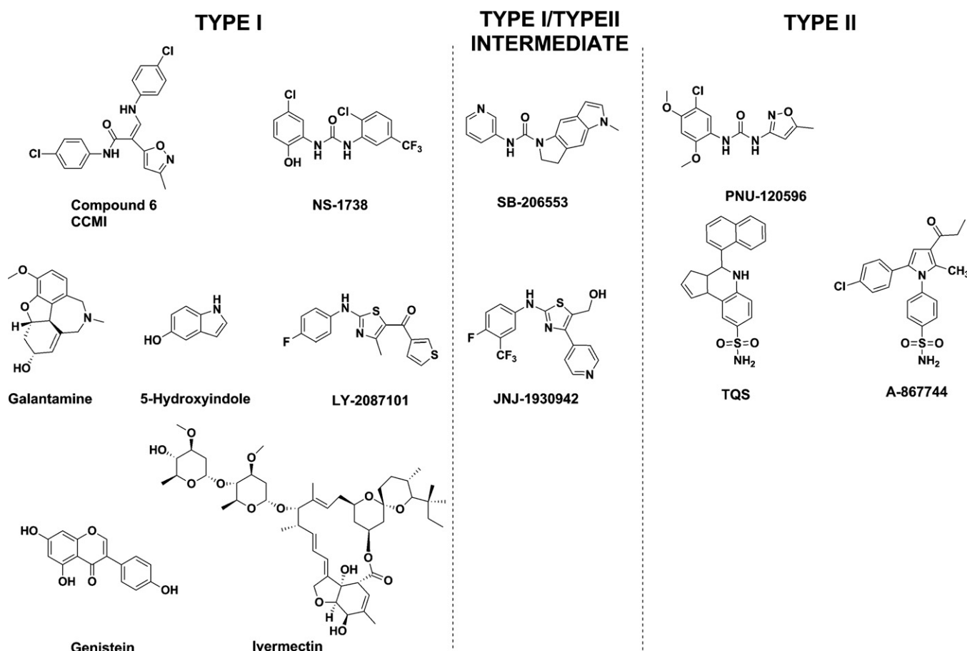
Fig. 2. Structures of \alpha 7 -active PAMs. The PAMs classified as type I, which increase the amplitude but do not strongly alter the kinetics of \alpha 7 -mediated agonist-evoked responses, are shown on the left. They include: CCM1, N-(4-chlorophenyl)- \alpha -[[(4-chloro-phenyl)amino]methylene]-3-methyl-5-isoxazoleacetamide; NS-1738, 1-(5-chloro-2-hydroxy-phenyl)-3-(2-chloro-5-trifluoromethyl-phenyl)-urea; Galantamine; 5-HI, 5-hydroxyindole; LY-2087101, [2-(4-fluoro-phenylamino)-4-methyl-thiazol-5-yl]-thiophen-3-yl-methanone; Genistein; and Ivermectin. Type II PAMs, which appear to slow or reverse \alpha 7 desensitization are shown on the right and include: PNU-120596, 1-(5-chloro-2,4-dimethoxy-phenyl)-3-(5-methyl-isoxazol-3-yl)-urea; TQS, 4-naphthalene-1-yl-3a,4,5,9b-tetrahydro-3-H-cyclopenta[c]quinoline-8-sulfonic acid amide; and A-867744, 4-(5-(4-chlorophenyl)-2-methyl-3-propionyl-1H-pyrrol-1-yl)benzenesulfonamide. PAMs proposed to be intermediate in their activity are shown in the center and include: JNJ-1930942, 2-[[4-fluoro-3-(trifluoromethyl)phenyl]amino]-4-(4-pyridinyl)-5-thiazolemethanol; and SB-206553, 3,5-dihydro-5-methyl-N-3-pyridinylbenzo [1,2-b:4,5-b']-di pyrrole-1(2H)-carboxamide.
